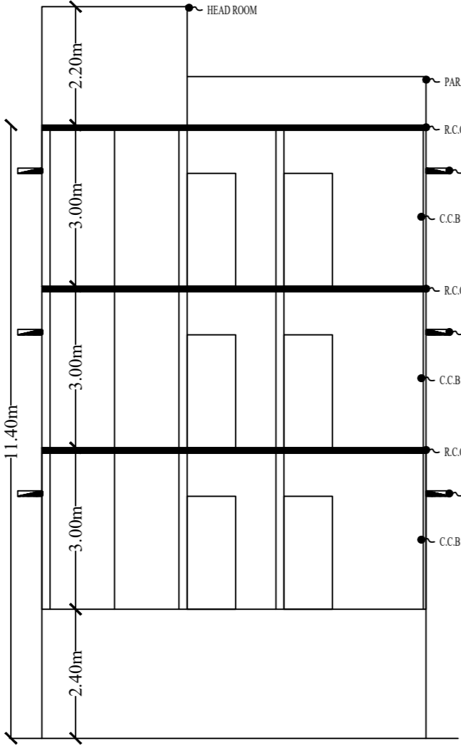
SECTION @ X-X'
